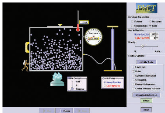
Figure 2 Particles in a box. In the ‘Gas Properties’ sim, pump the handle to add heavy or light particles to the box and see them move about, colliding with each other and the walls. Cool the box with ‘ice’ and see the particles’ motion slow as the thermometer and pressure-gauge readings fall. Increase gravity and see a pressure gradient form. The companion ‘Balloons and Buoyancy’ sim explains the microscopic origin of buoyancy through hot air and helium balloons.
