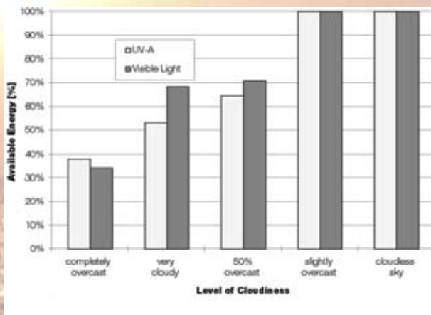
Figure 10: Losses of available solar energy at different weather conditions [16]
